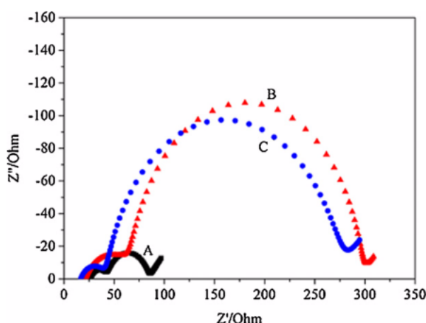
Fig. 8. Electrochemical impedance spectra of DSCs: (A) N719, (B) rutin, and (C) mangosteen pericarp extracts.
